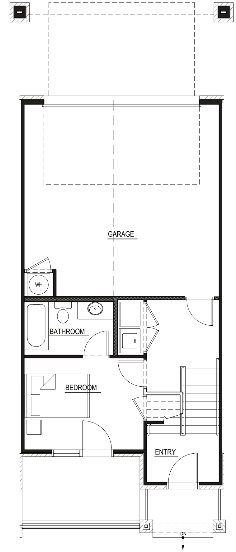
UNIT A FIRST FLOOR PLAN
